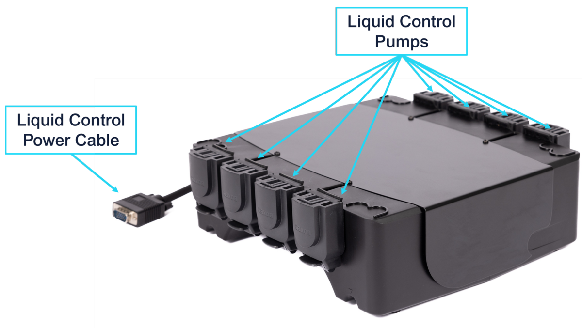
Figure 4: Liquid Control Module
