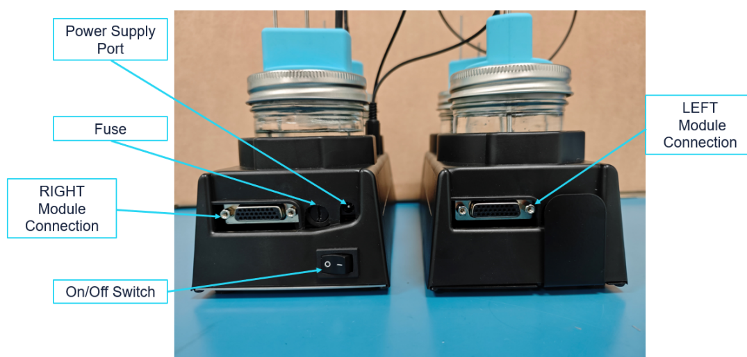
Figure 20: Rear view of the Pre-Humidifier units. Note the power switch is only present on one side. Please ensure the units are connected to each other before powering on.
