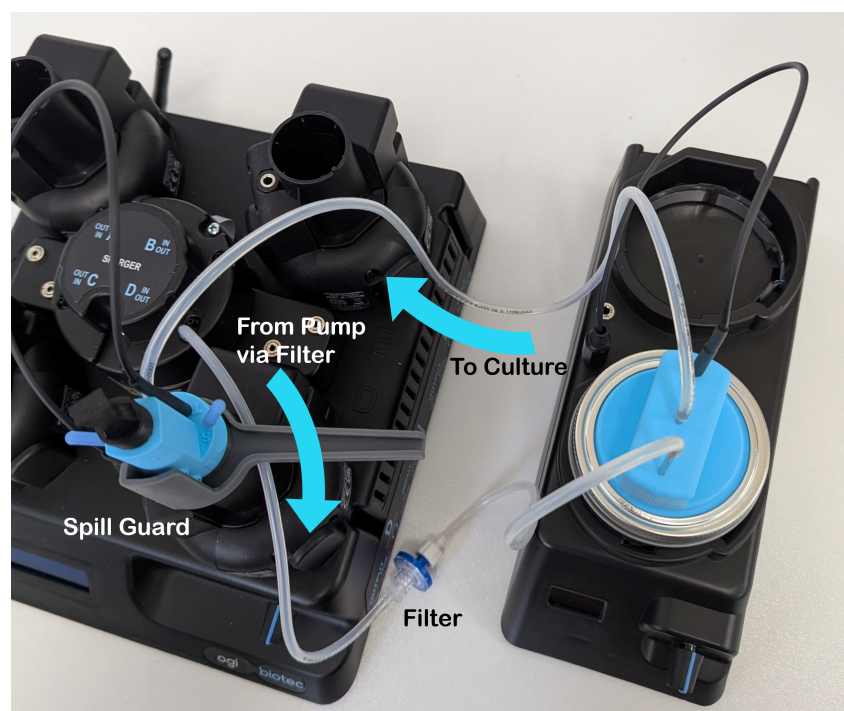
Figure 24: Pre-humidifier unit with jar in slot D connected to culture flask in Reactor D. Pathway of airflow is highlighted, and filter and spill-guard is attached.
