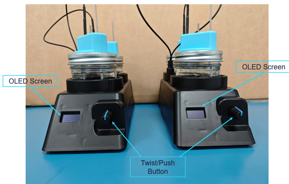
Figure 19: Front view of the Pre-Humidifier units
