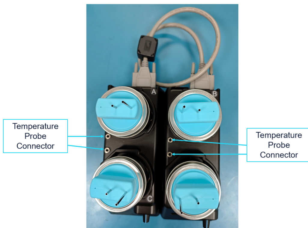
Figure 21: Top view of the Pre-Humidifier units. There are four connectors for the temperature probes
