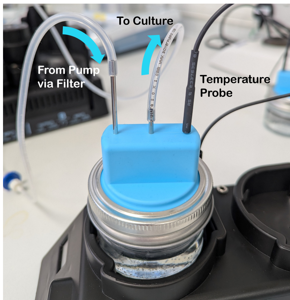
Figure 22: Connection of the pre-humidifier flasks. Ensure that the pump connects ONLY to the long needle, not the short needle. Improper connection will lead to water being pumped into the culture flask, filling it quickly and leading to spillage.
